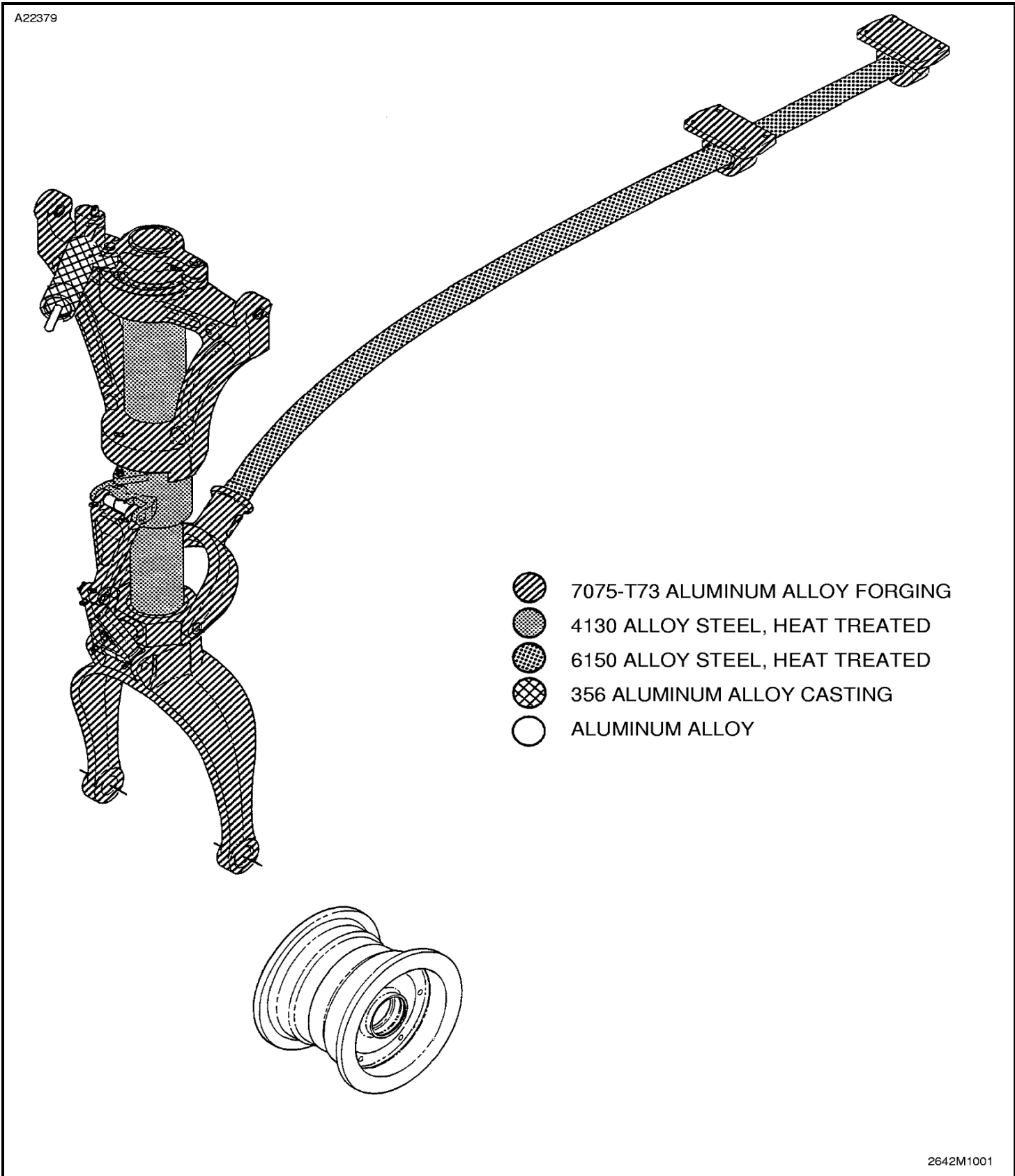
Figure 701 : Sheet 1 : Nose Landing Gear Construction Materials
